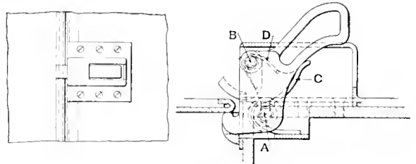
Foot-Operated Trap Door Latch Which Insures the Opening of the Door
